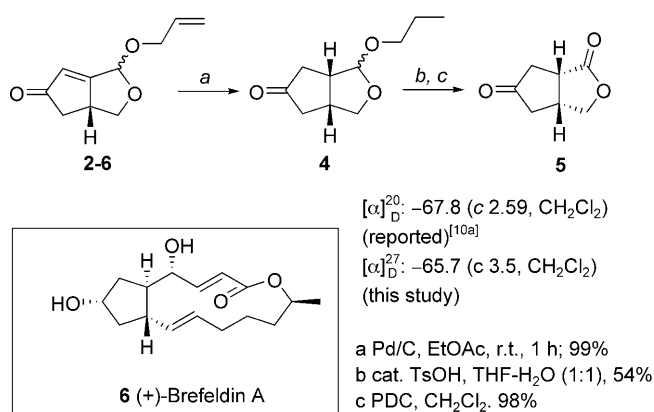
Scheme 2. Further functionalization of 2-6 .
