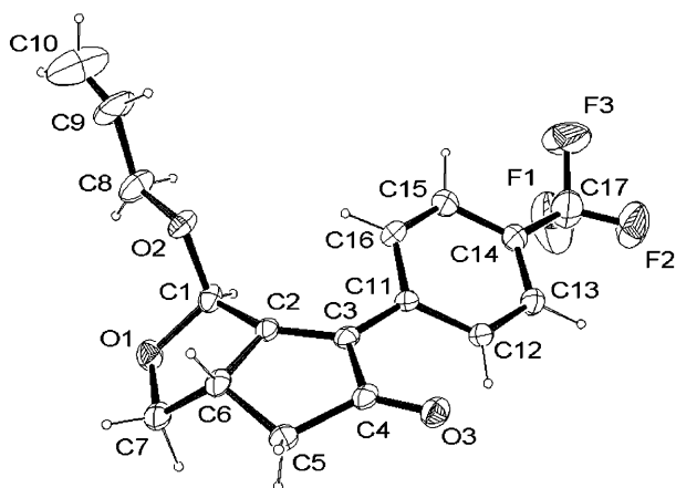
Figure 1. ORTEP drawing of 2-5a .
