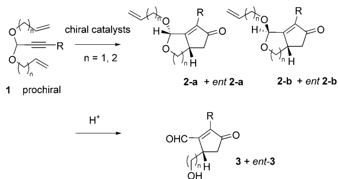
Scheme 1. Asymmetric desymmetrization of bisallyl propargyl acetals
